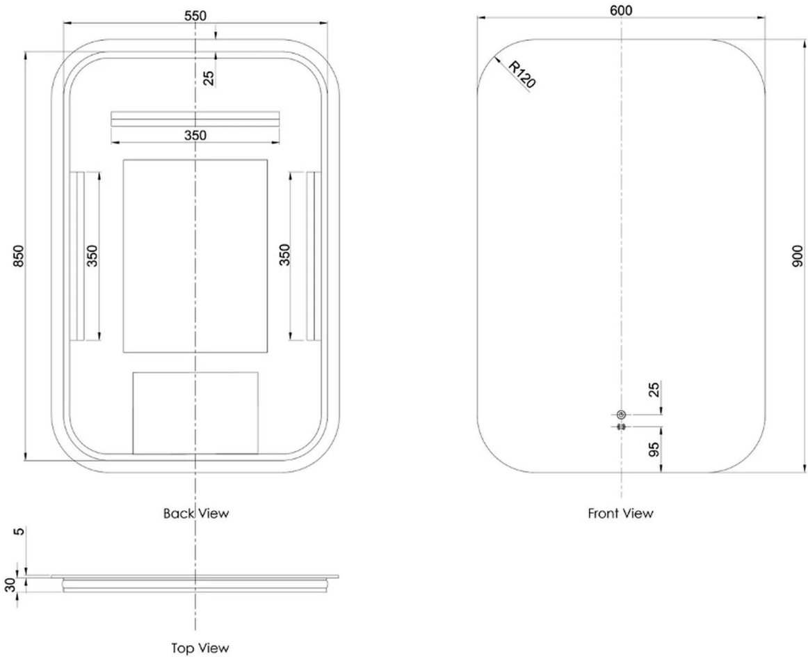
Front, side and back views - measurements in millimetres
