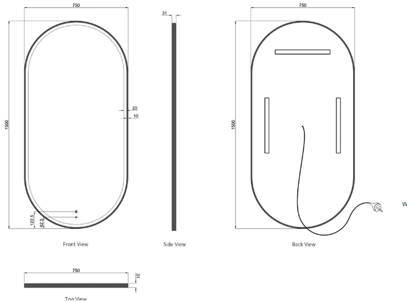
Front, side and back views - measurements in millimetres
