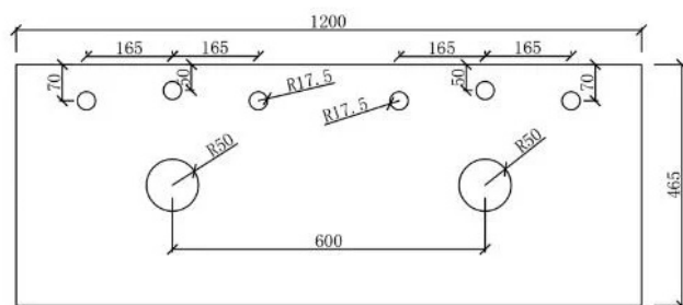
Back View Pre Semi-Drilling Taphole
