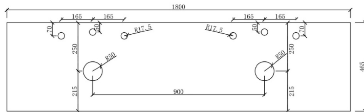
Back View Pre Semi-Drilling Taphole
