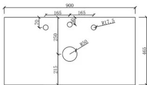
Back View Pre Semi-Drilling Taphole
