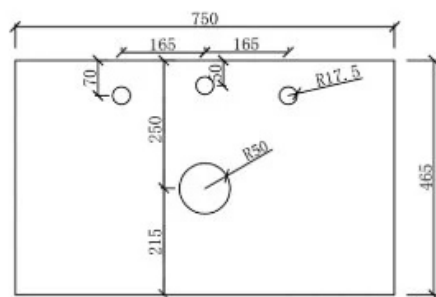
Back View Pre Semi-Drilling Taphole
