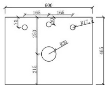
Back View Pre Semi-Drilling Taphole
