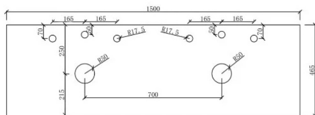
Back View Pre Semi-Drilling Taphole
