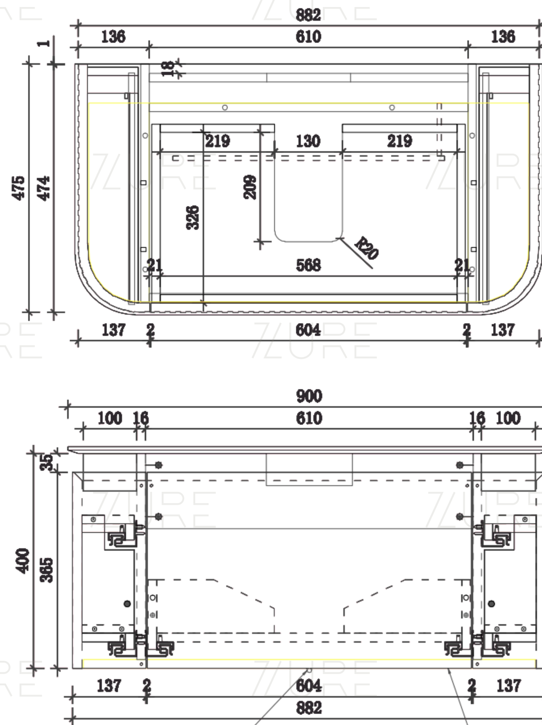
Front View
