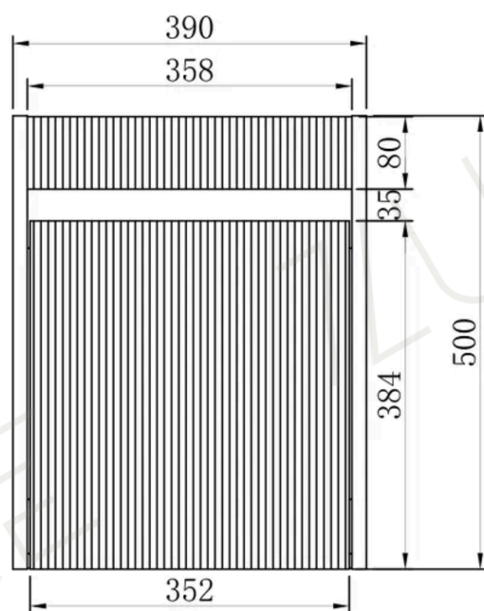
Front View
