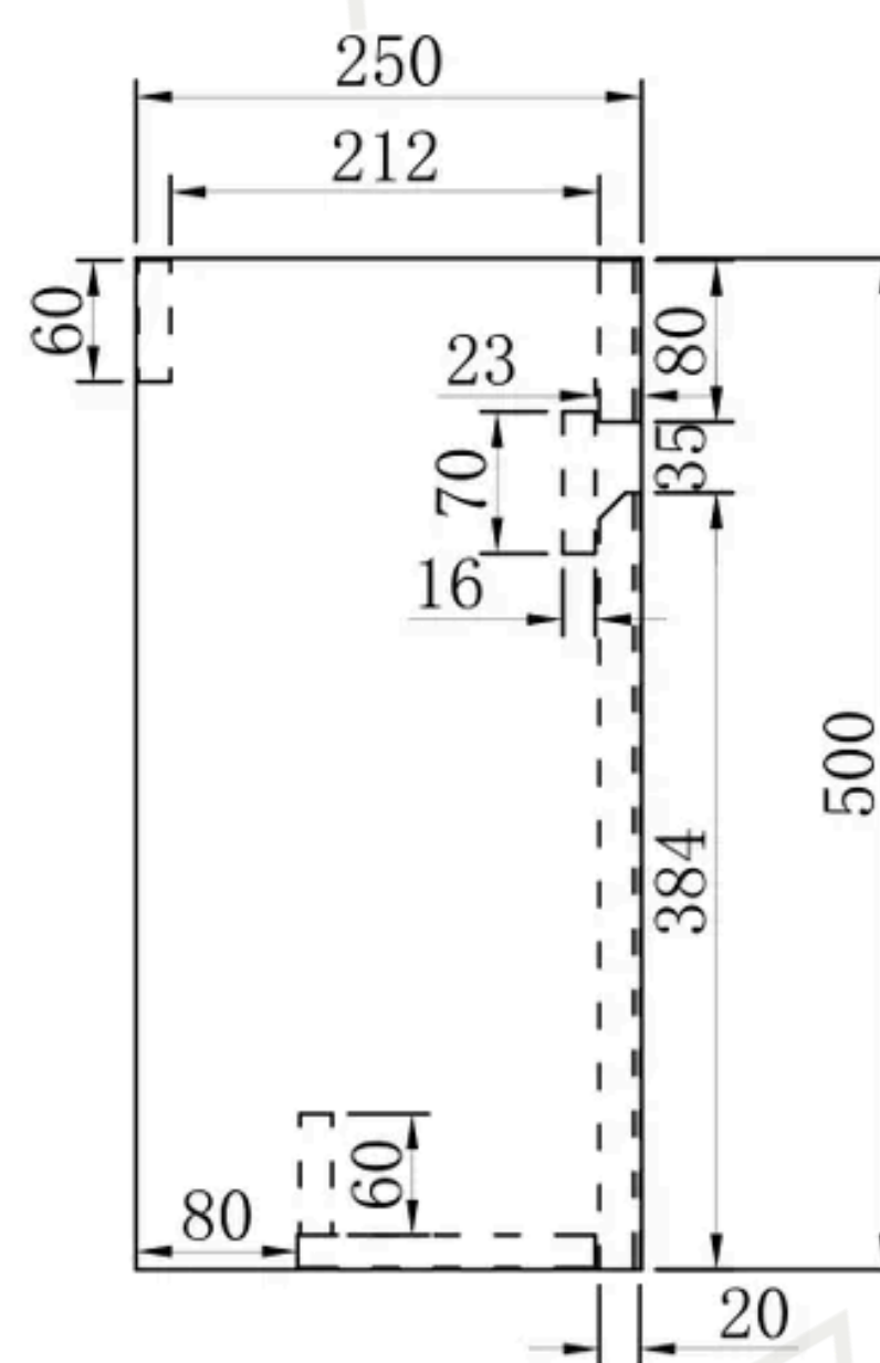
Side View
