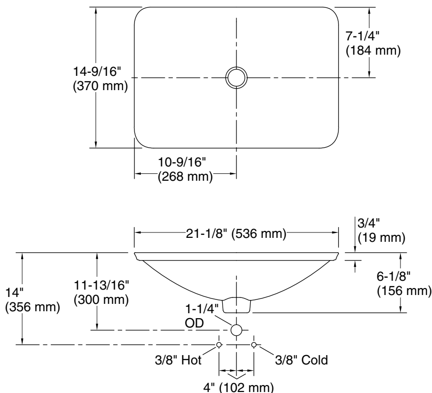
Standard Installation
