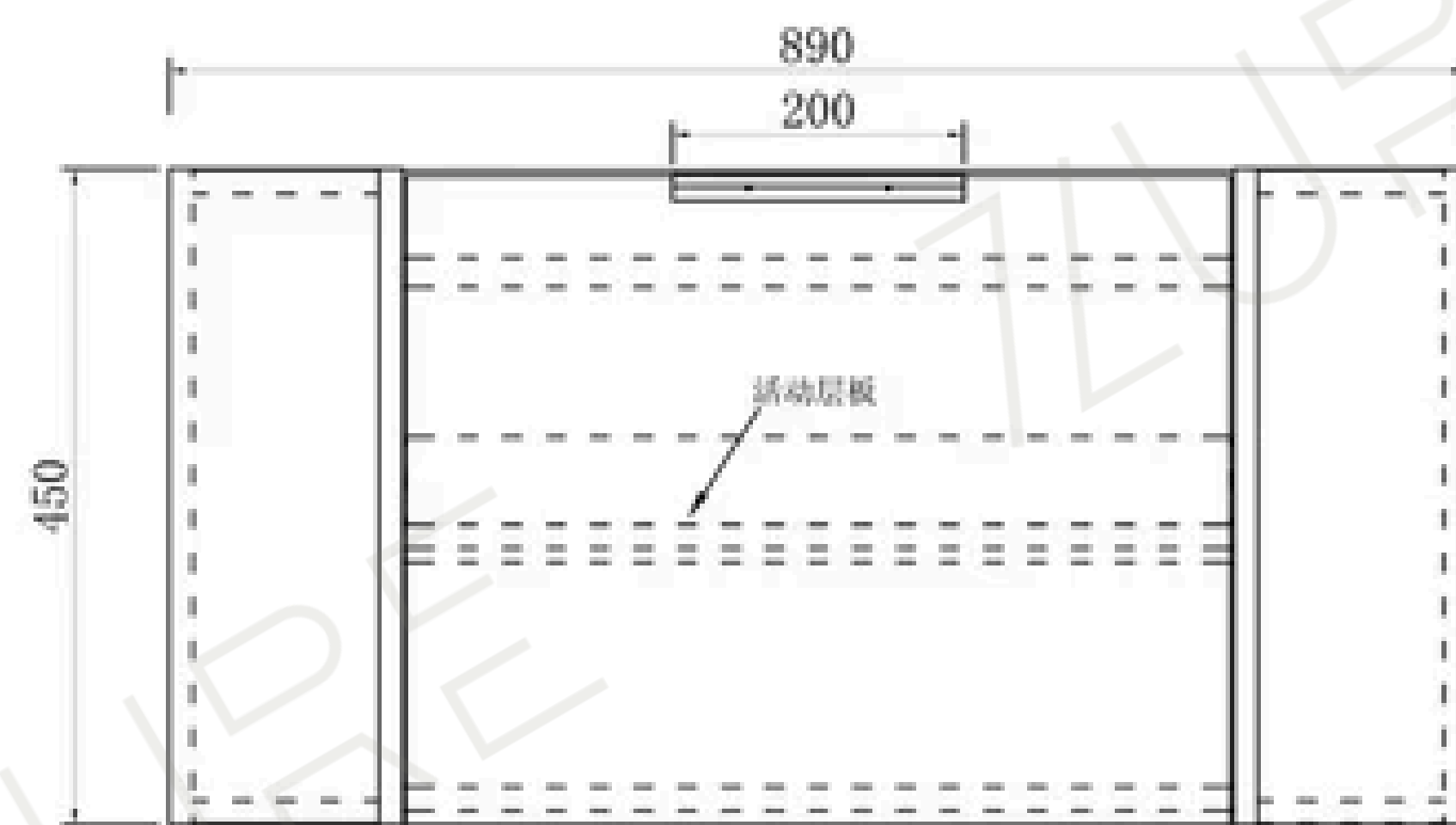
Front View
