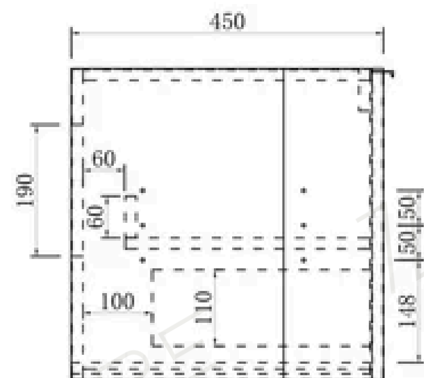
Side View
