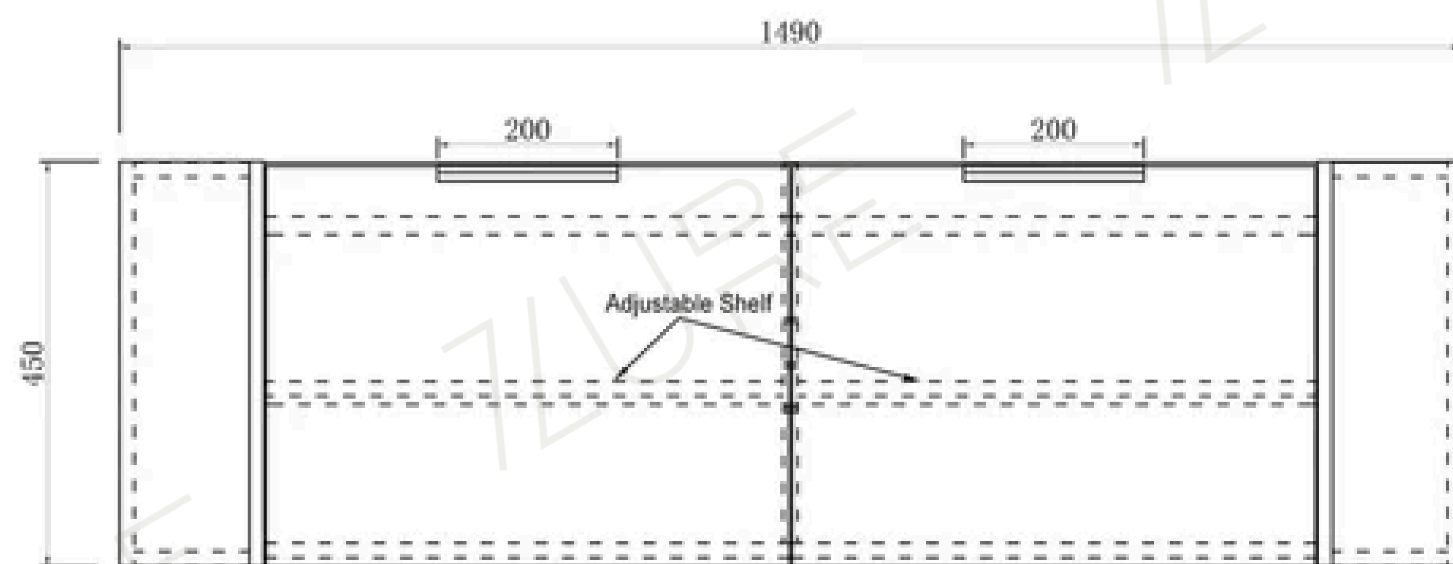
Front View
