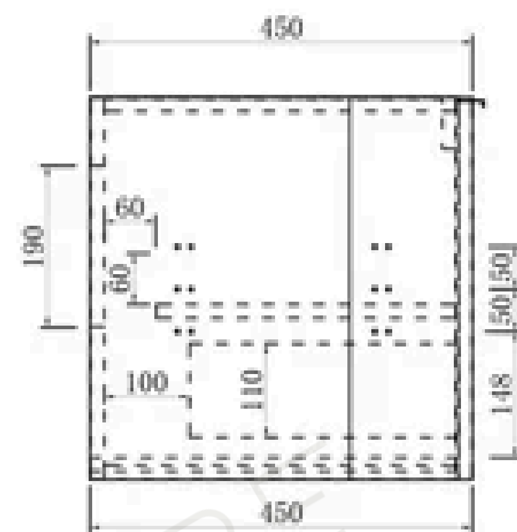
Side View
