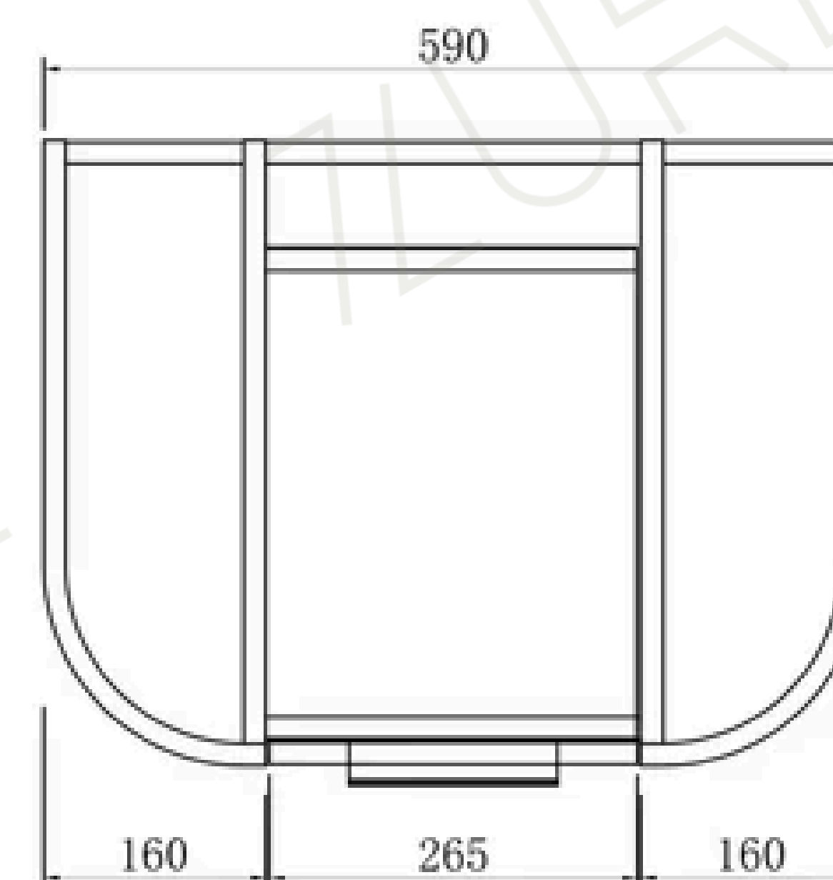
Top View
