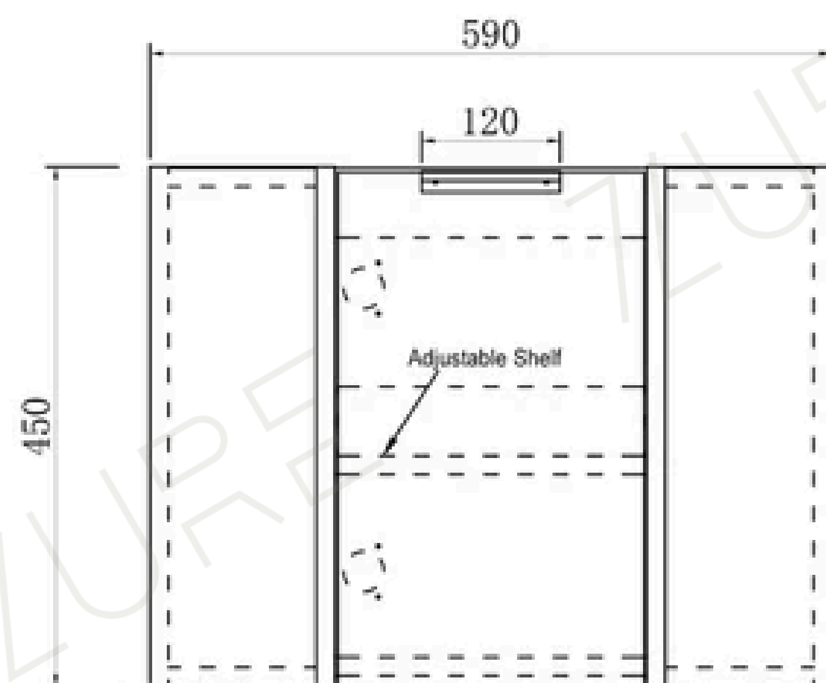
Front View
