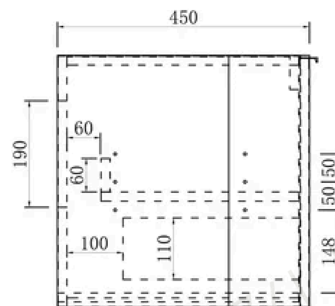
Side View
