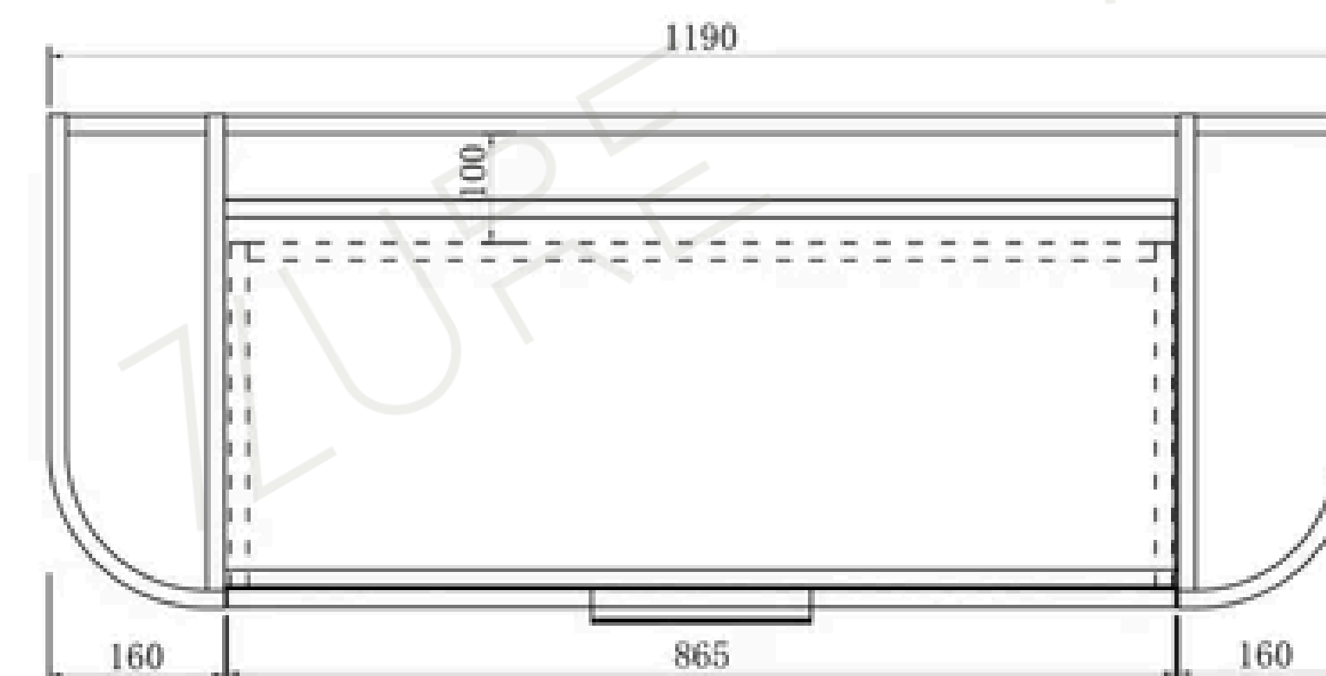
Top View
