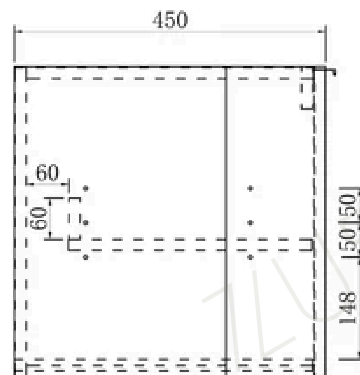
Side View
