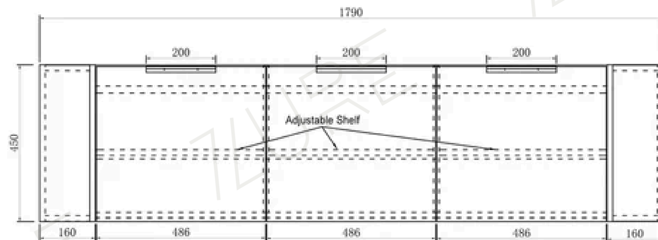
Front View
