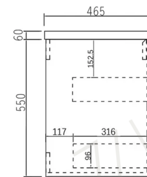
Side view
