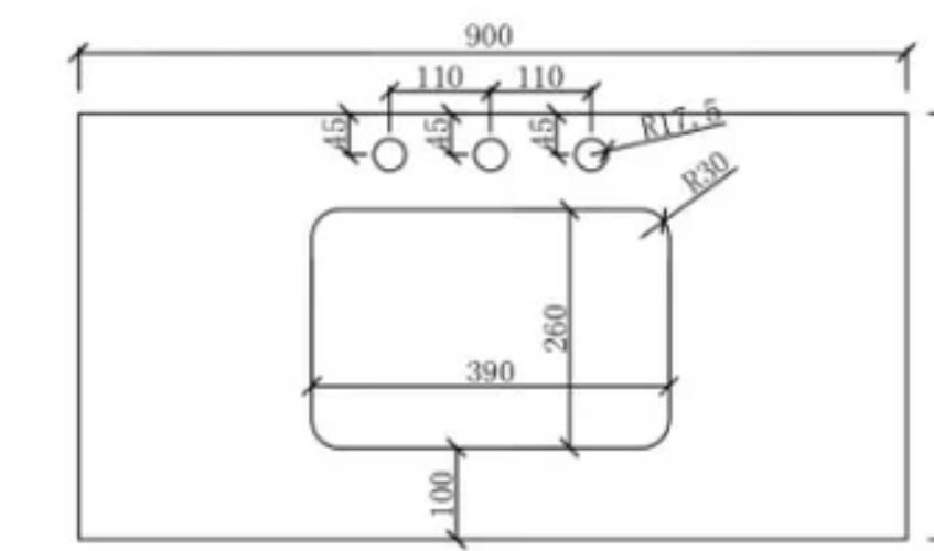
Back View
